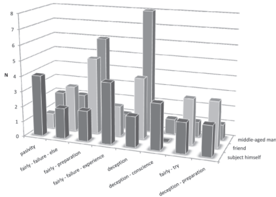
Graph 4 Solutions of "job-situation": Comparison of actor's positions
